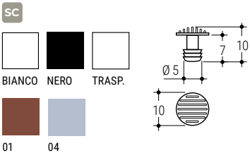
121 B Paracolpo morbido testa zigrinata Soft bumper with knurled head
