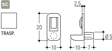
196 Reggicristallo trasparente per cristalli da 4 a 6 mm Glass shelf support, plastic clear for glass shelf thickness from 4 to 6 mm
