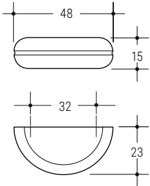
319 48x15 h 23 i 32 VE VS VG VM VR KU SP
