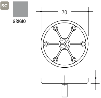
761S Piedino Ø 70 h 8 v. 8MAx20 Bearing Ø 70 h 8 v. 8MAx20 500 Pz
