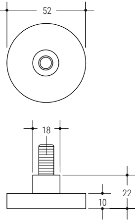
709B Ø 52 h 22 v. 10MA VE VS VG VM MT SP
