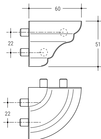
1766B 60x51 i 22 VE VS VG KU GA
