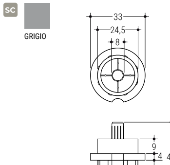
726 Piedino reg. Ø 24,5/33 h 42 Reg. bearing Ø 24,5/33 h 42 200 Pz
