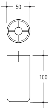
744 Ø 50 h 100 v. B2 VE VS VG VM MT KU SP
