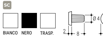
113 A Paracolpo a pressione testa morbida Pressur-shock absorber with soft head
