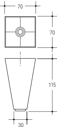
758R Regolabile - Adjustable 30x30/70x70 h 115 v. A2 VE VS VG MT KU SP
