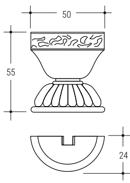
1643 50x55 h 24 VE VS VG KU GA
