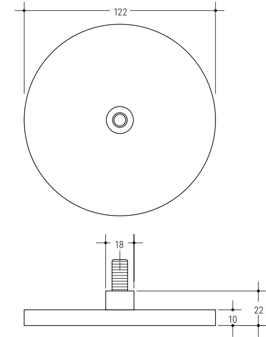
715 Ø 122 h 22 v. 10MA VE VS VG VM MT SP
