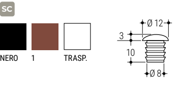
121 Paracolpo morbido Soft bumpers
