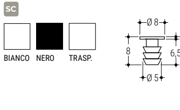
121 D Paracolpo morbido testa liscia Soft bumper with smooth head
