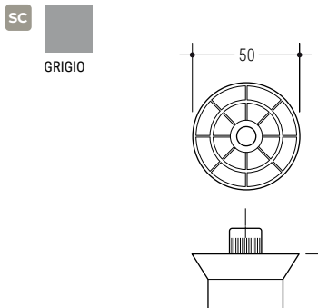
718 Piedino reg. Ø 34/50 h 35 Reg. bearing Ø 34/50 h 35 200 Pz
