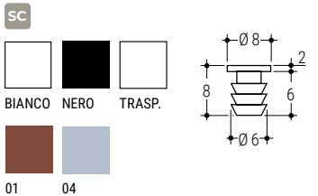
121 C Paracolpo morbido testa liscia Soft bumper with smooth head
