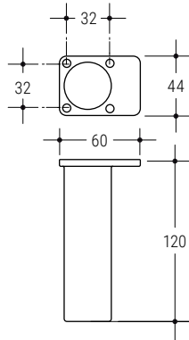
716 Ø 35 44x60 flangia/flange h 120 VE VS VG MT SP
