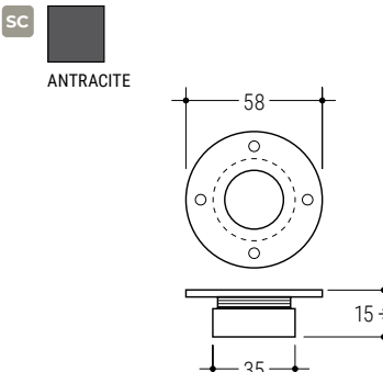
738 Piedino reg. Ø 58/35 h 15/20 Reg. bearing Ø 58/35 h 15/20 600 Pz
