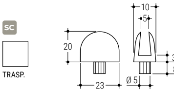
159 Z TRASPARENTE Reggicristallo trasparente Transparent glass support
