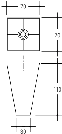
758 30x30/70x70 h 110 v. B2 VE VS VG MT KU SP
