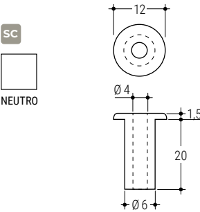
1890 Rondella salva specchi Mirror protecting washer
